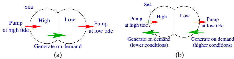
Figure G.12. Different ways to use the tidal pumping trick. Two lagoons are located at sea-level. (a) One simple way of using two lagoons is to label one the high pool and the other the low pool; when the surrounding sea level is near to high tide, let water into the high pool, or actively pump it in (using electricity from other sources); and similarly, when the sea level is near to low tide, empty the low pool, either passively or by active pumping; then whenever power is sufficiently valuable, generate power on demand by letting water from the high pool to the low pool. (b) Another arrangement that might deliver more power per unit area has no flow of water between the two lagoons. While one lagoon is being pumped full or pumped empty, the other lagoon can deliver steady, demand-following power to the grid. Pumping may be powered by bursty sources such as wind, by spare power from the grid (say, nuclear power stations), or by the other half of the facility, using one lagoon's power to pump the other lagoon up or down.
