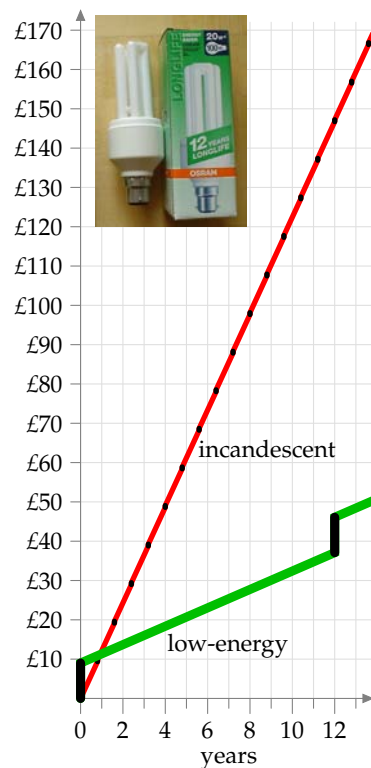
Figure 9.3. Total cumulative cost of using a traditional incandescent 100 W bulb for 3 hours per day, compared with replacing it now with an Osram Dulux Longlife Energy Saver (pictured). Assumptions: electricity costs 10p per kWh; replacement traditional bulbs cost 45p each; energy-saving bulbs cost £9. (I know you can find them cheaper than this, but this graph shows that even at £9, they're much more economical.)
