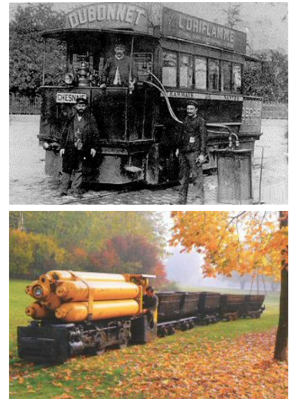
Figure 20.24. Top: A compressed-air tram taking on air and steam in Nantes. Powering the trams of Nantes used 4.4 kg of coal (36 kWh) per vehicle-km, or 115 kWh per 100 p-km , if the trams were full. [5qhvcb] Bottom: A compressed-air locomotive; weight 9.2 t, pressure 175 bar, power 26 kW; photo courtesy of Rüdiger Fach, Rolf-Dieter Reichert, and Frankfurter Feldbahnmuseum.
